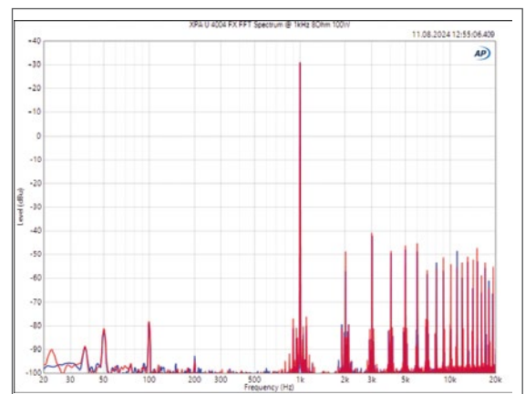
FFT spectrum
