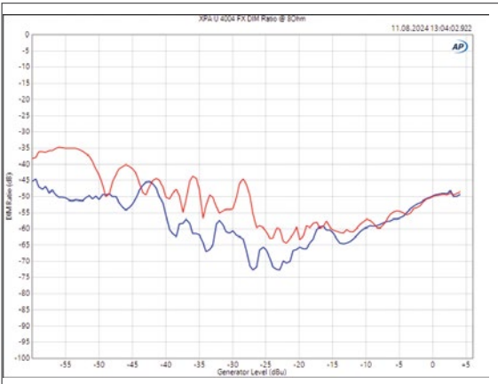
Fig. 10: Transient intermodulation distortion (DIM100) for Ch1 (blue) and Ch2 (red) as an example depending on the input level measured at a 4×8-Ω load. The curve is unusually unstable.
