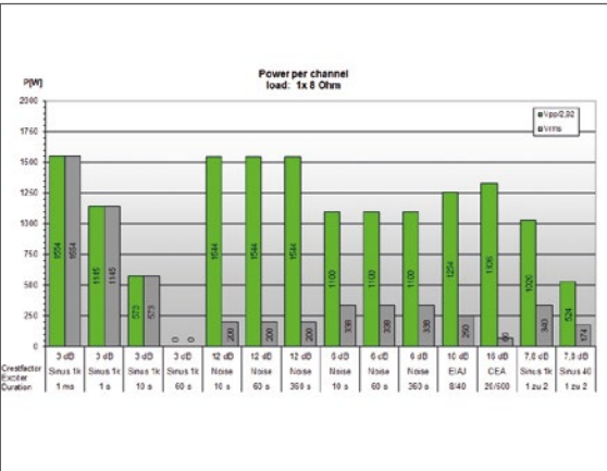
Fig. 11: Performance values of the XPA U 4004 FX an 8 Ω with single channel loading with different signal types. See text for details.
