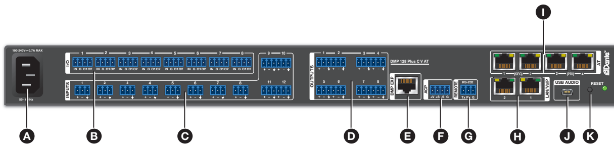
Figure 1. DMP 128 Plus Rear Panel
