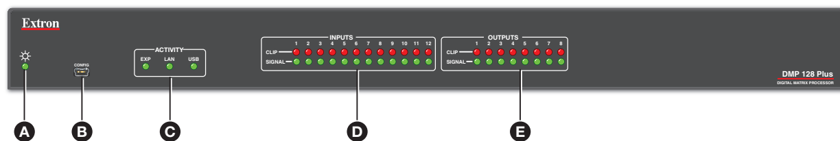
Figure 2. DMP 128 Plus Front Panel
