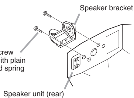
[Horizontal speaker installation]
