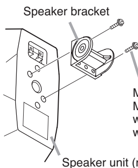
[Vertical speaker installation]
